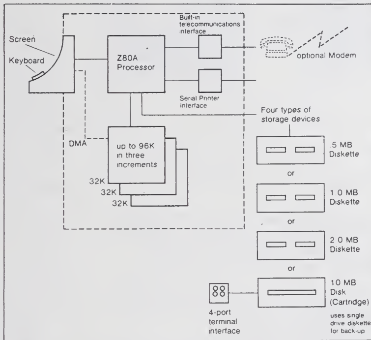
Datapoint 1550 System Architecture
